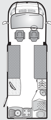
AIRSTREAM 630 EK
