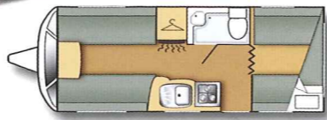
Zenith 5 - 5 Berth
