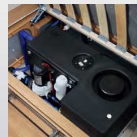
30 litre internal fresh water tank in twin axle models with additional pump for tank filling or direct feed to taps
